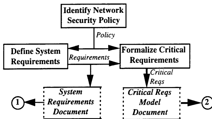
Figure 3: Requirements Documentation
