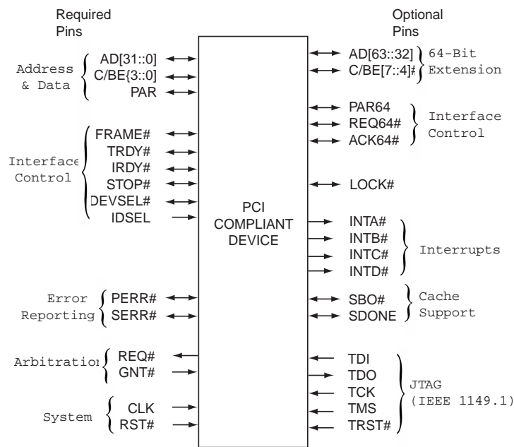
Figure 1: PCI Compliant Device Signals
